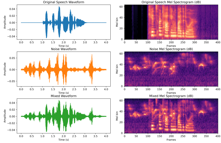
Figure 3.9: Example of adding natural_soundscape(chirping_birds) noise to a sample in RAVDESS
