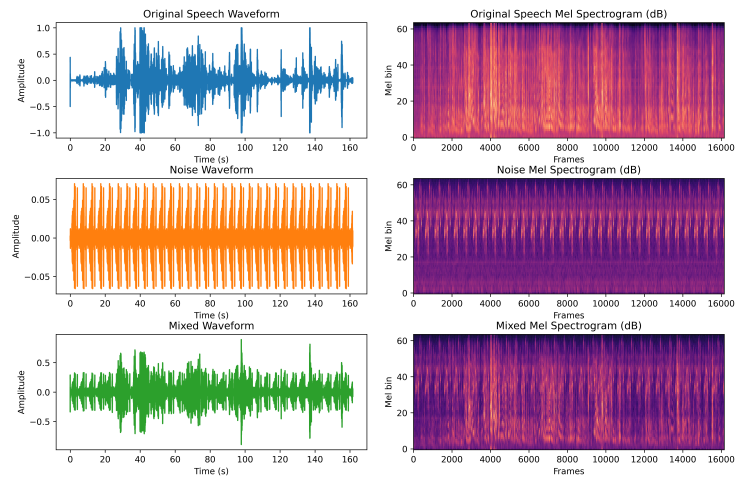
Figure 3.10: Example of adding natural_soundscape(chirping_birds) noise to a sample in IEMOCAP
